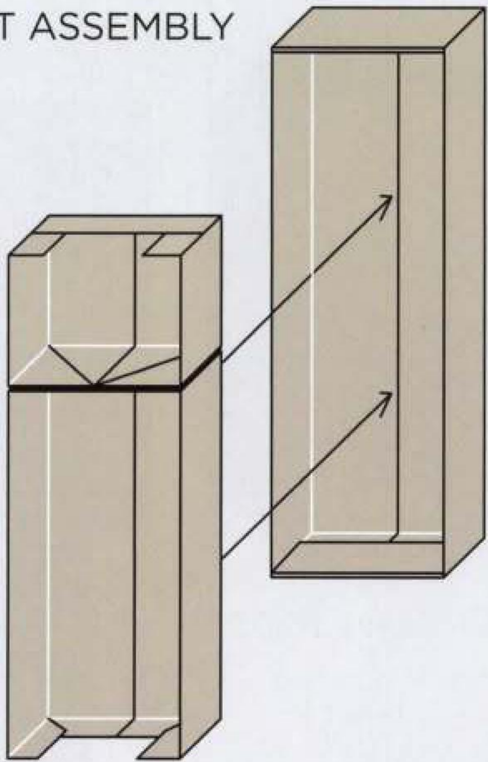
1. Insert Part 2 into Part 1 as the arrows indicate
